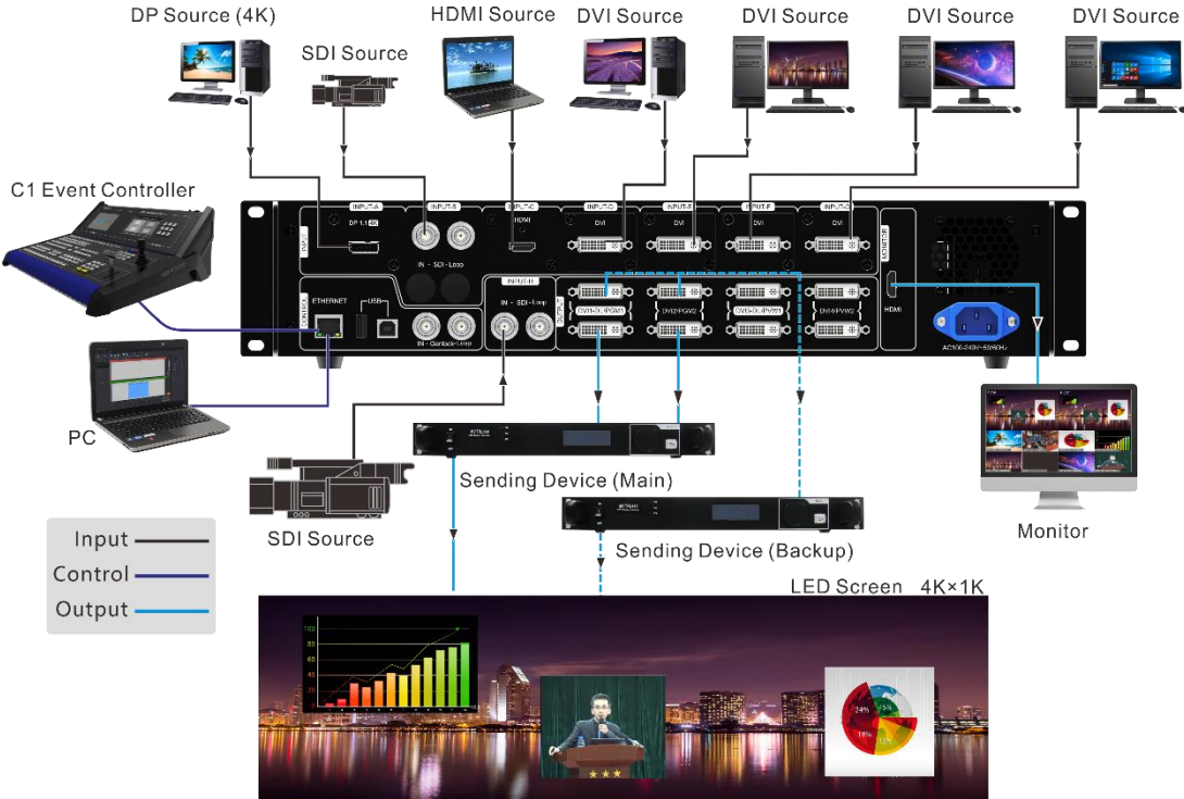
Figure 3-2 Connections for Switcher mode
